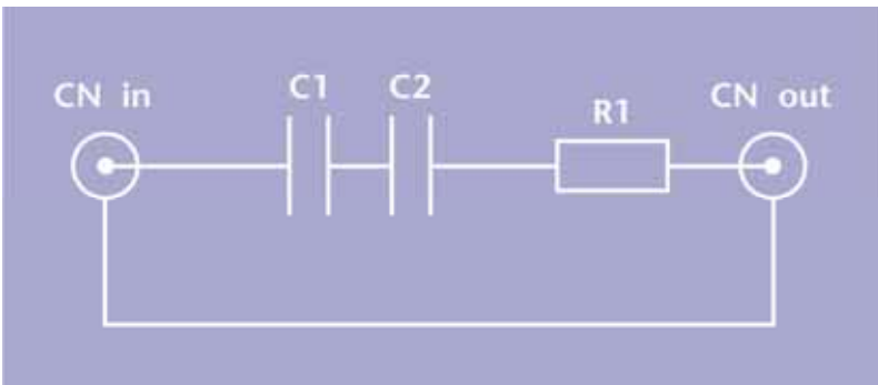
Figure 6. High frequency RF barrier
